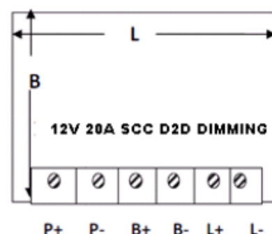
Solar Charge Controller-D2D with Dimming
